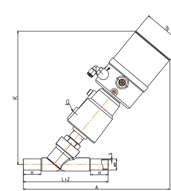
125 Series Welded connection
