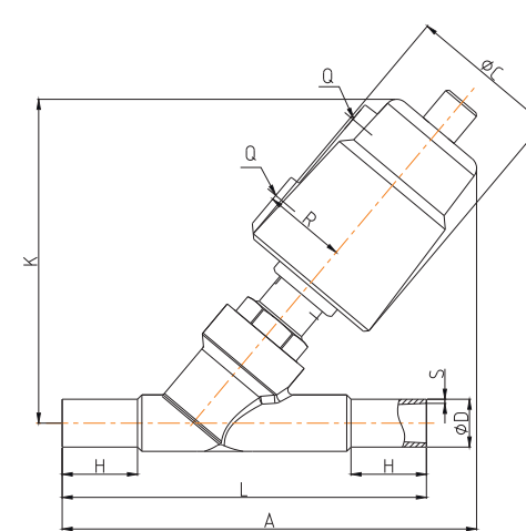
Welded Connection
