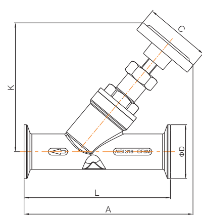
Tri-clamp connection
