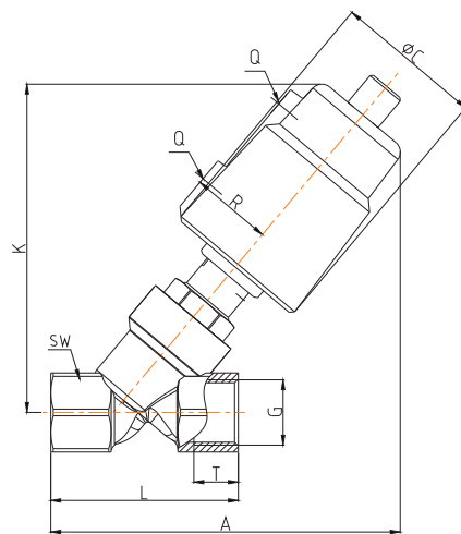
Threaded Connection
