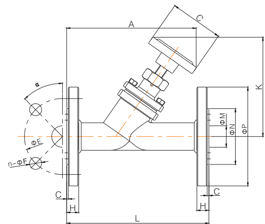
Flange connection
