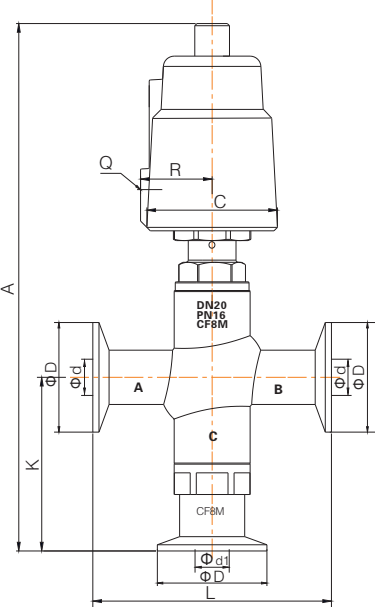
Tri-clamp connection
