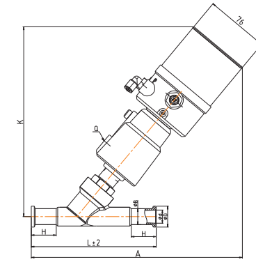
125 Series Tri-clamp connection
