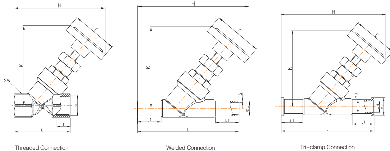
Threaded Connection
