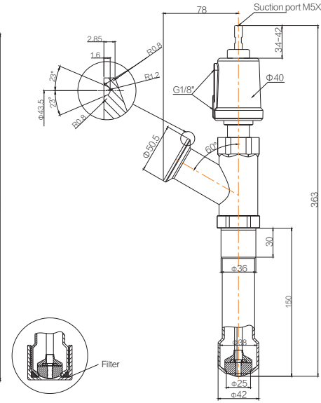
1AM Filling valve with internal sealing and filter
